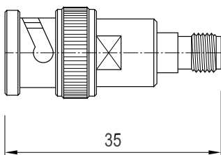
SMA Plug to BNC Plug
