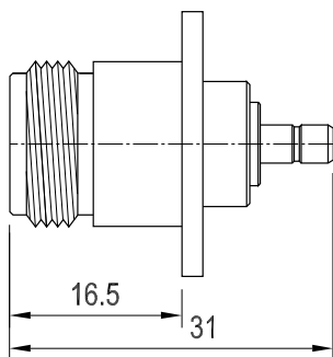
SMB Jack to N Jack
