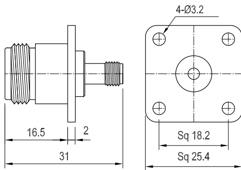
SMA Jack to N Jack
