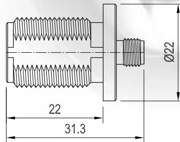
SMA Jack to N Jack
