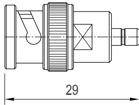
SMB Jack to BNC Plug
