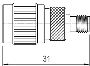
SMA Jack to TNC Plug
